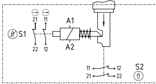
EX-AZM 415-02/02ZPK...-3D
