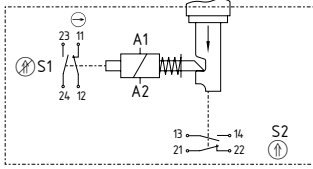
EX-AZM 415-11/11ZPK...-3D
