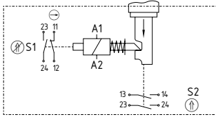
EX-AZM 415-11/20ZPK...-3D
