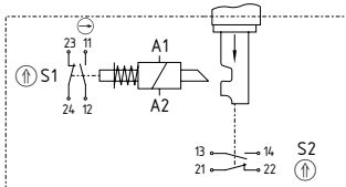
EX-AZM 415-11/11ZPKA...-3D
